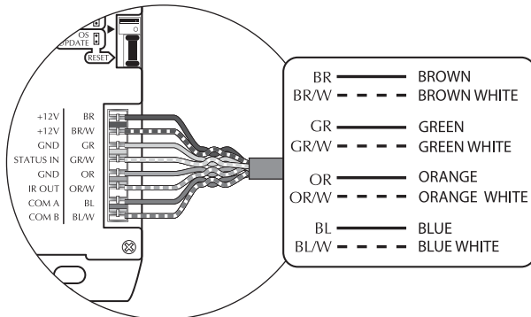
CAT-5 to UNO - Connection
